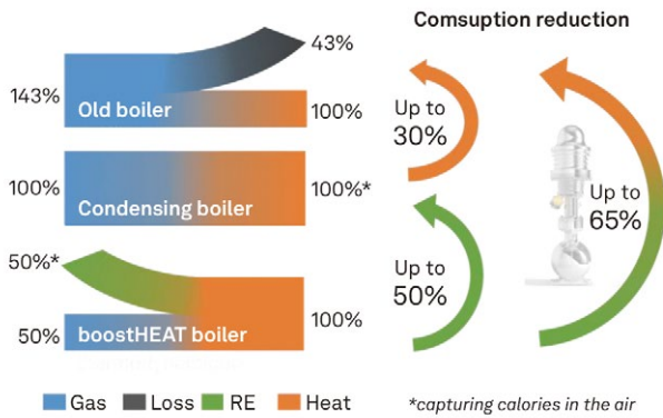
Figure 2: the BoostHEAT heat pump boiler versus alternative boiler types
