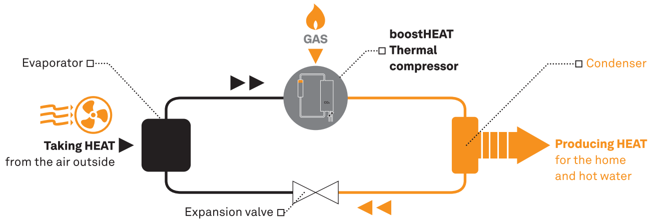
Figure 1: the BoostHEAT heat pump boiler principle
