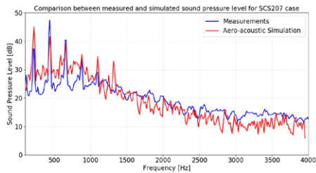
Fan noise application. Correlation between Actran AeroAcoustics predictions and measurements. Model & results courtesy of John Deere
