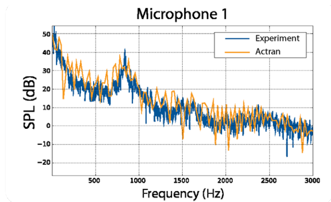
Sound pressure level of air conditioning duct. Correlation between Actran AeroAcoustics predictions and measurements. Model & results courtesy of Visteon
