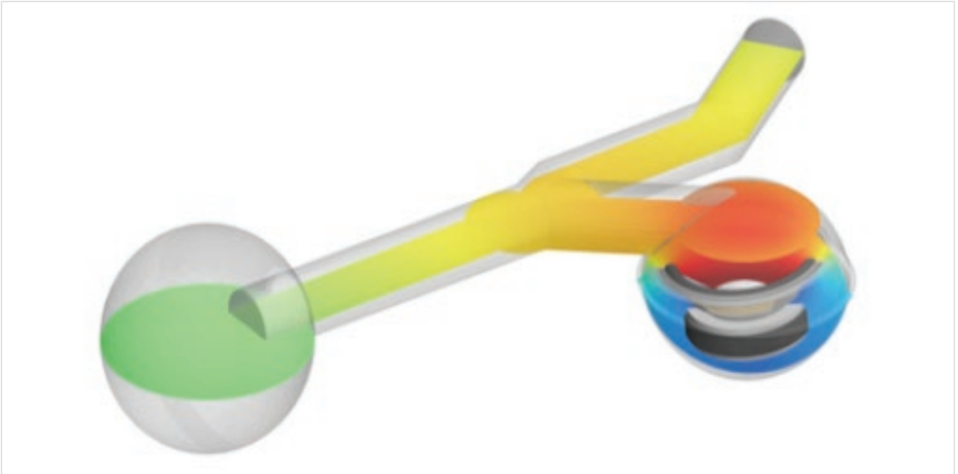
Exhaust acoustic pressure cancellation
